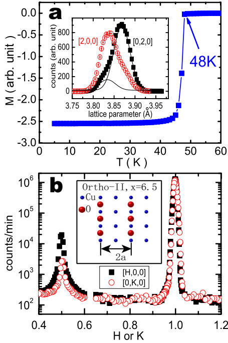
FIG. 1. (Color online) (a) The temperature dependence of the magnetic susceptibility showing an onset T_c of 48 K with width of 2 K. The inset shows (2,0,0) and (0,2,0) Bragg peaks indicating a detwinning ratio of 85%, as illustrated by the two fitted Gaussian lines for (0,2,0) peak. (b) The ortho-II oxygen ordering (1/2, 0, 0)/(0, 1/2, 0) and nuclear (1, 0, 0)/(0, 1, 0) peaks. Since the CuO chains form the ortho-II superstructure as shown in the inset, scattering along the a^* direction should result in the (1/2, 0, 0) peak.
