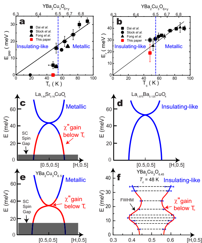
FIG. 7. (Color online) (a) Spin gap energies as a function of T_c for YBCO. There is a sudden reduction below y=0.5 and the MIC. (b) The resonance energies and their widths as a function of T_c for YBCO. The energy width of the resonance increases dramatically below y=0.5 and the MIC. (c) The schematic dispersion for optimally doped \text{La}_{1.84}\text{Sr}_{0.16}\text{CuO}_4 . On cooling below T_c , a clean spin gap (about 6 meV) opens and the spectral weight shifts from below to above the gap, as shown in red region (Refs. 12 and 13). (d) The schematic dispersion for static stripe ordered \text{La}_{1.875}\text{Ba}_{0.125}\text{CuO}_4 , where incommensurate spin fluctuations extend to zero energy and there is no spectral weight enhancement below T_c (Refs. 17 and 18). (e) Dispersion of YBCO for y \geq 0.5 . The low-energy incommensurate scattering were obscured by the presence of the low-temperature spin gap. The lines within the gap indicate the expected dispersion from a naive stripe model for y < 0.5 samples (Ref. 5). (f) Observed dispersion for \text{YBa}_2\text{Cu}_3\text{O}_{6.45} along the a^* direction. The part above 12 meV is consistent with an hourglasslike dispersion, which breaks down at low energies.
