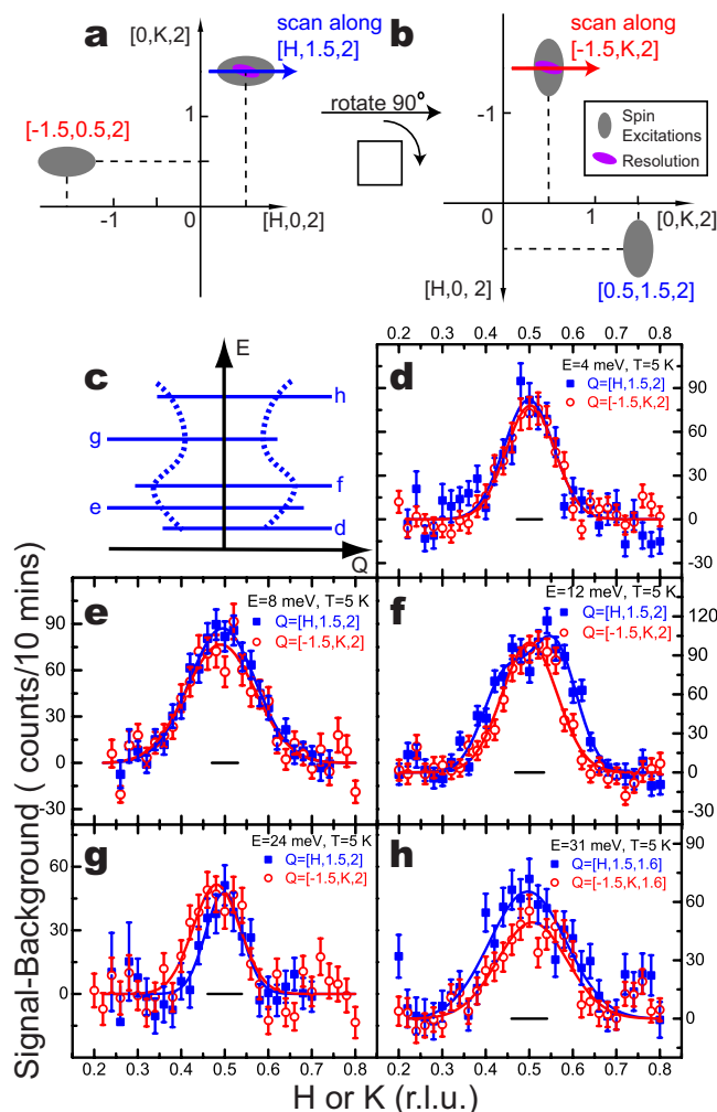
FIG. 6. (Color online) [(a) and (b)] Experimental setup for studying magnetic anisotropy in our \text{YBa}_2\text{Cu}_3\text{O}_{6.45} . The measurements were carried out in the [H, K, 4K/3] and [H, K, 4H/3] zones by rotating the sample 90 degrees along the c^* axis. The advantage of such a setup is that the instrumental resolutions are identical in the a^* and b^* scan directions. (c) Schematic Q scans at different energies. [(d)–(h)] Q -scans along the [H, 1.5, 2] and [-1.5, K, 2] directions at different energies in the low-temperature superconducting state. While the scattering profiles are commensurate and isotropic at 4 and 8 meV, clear anisotropic scattering appears at 12 meV. The data show clear flattish top. The Q profiles become narrow and isotropic again near the resonance energy. The instrumental resolutions are shown as the horizontal bars.
