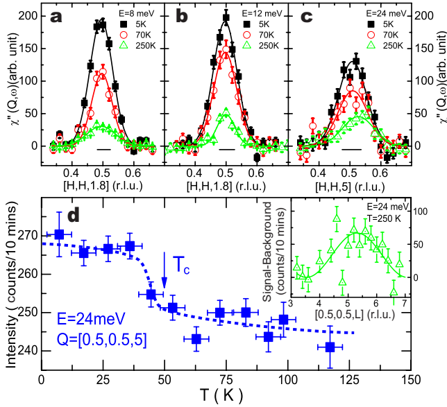
FIG. 5. (Color online) [(a)–(c)] Wave vector dependence of dynamic susceptibility along the [H, H] direction at different energies and temperatures. There are clear magnetic scattering consistent with acoustic magnetic scattering structure factor even at 250 K, as shown in the inset of (d). (d) The temperature dependence of the scattering at 24 meV and (0.5, 0.5, 5) shows an order-parameterlike increase below T_c , a hallmark of the resonance.
