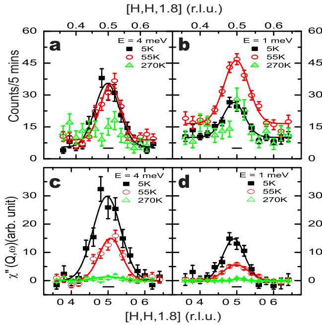
FIG. 2. (Color online) Q scans along the [H,H,1.8] direction at (a) \hbar\omega=4 meV and (b) 1 meV. While the intensity at 4 meV shows no sign of temperature dependence, the intensity at 1 meV clearly increases when the system changes from 5 to 55 K. The corresponding \chi''(Q,\omega) are shown in (c) and (d), respectively. The horizontal bars are the instrumental resolutions.
